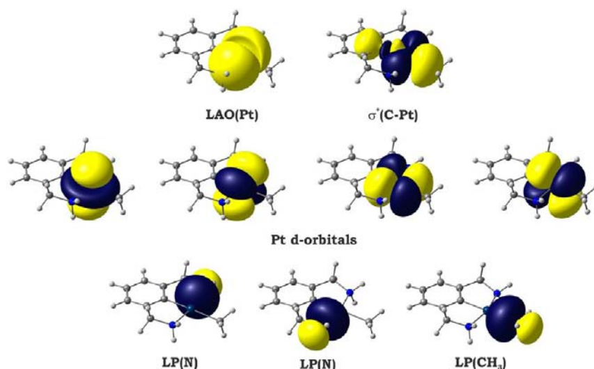
Figure 5. Selected NBOs of van Koten metal fragment [L(CH_3)Pt] .
