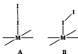
Figure 1. X-ray structures (hydrogen atoms are omitted for clarity) of adducts of I_2 investigated by (a) G. van Koten et al., 2 complex 1, (b) F. A. Cotton et al., 3 complex 2, (c) D. W. Shaffer et al., 4 and (d) R. Makiura et al. 5 (cationic species, counterion not shown). For compounds in (a) and (b), ChemDraw schematic representations are also given.
