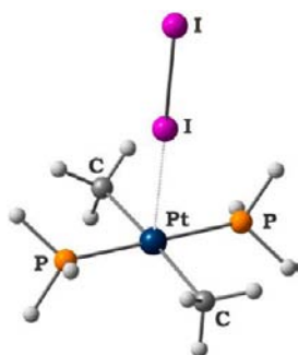
Figure 13. Equilibrium geometry configuration of the model adduct [(\text{CH}_3)_2(\text{PH}_3)_2\text{Pt}\cdot\text{I}_2] .
