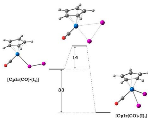
Figure 18. Schematic energy diagram (in kcal/mol) for the oxidative addition process [\text{CpIr}(\text{CO})\cdot(\text{I}_2)] \rightarrow [\text{CpIr}(\text{CO})\cdot(\text{I})_2] .
