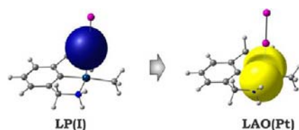
Figure 7. The major contributor to the (I_2) \rightarrow M interaction in an NBO analysis (for Y = CH 3 ).
